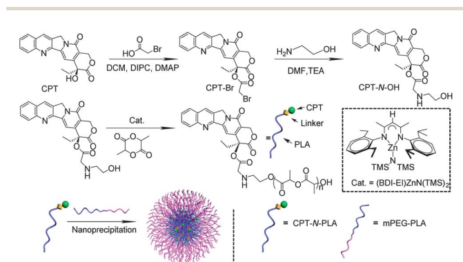
Fig. 1 Preparation of PEGylated CPT- N -PLA NCs via CPT- N -OH initiated LA polymerization in the presence of (BDI-EI)ZnN(TMS) 2 , followed by nanoprecipitation and non-covalent surface modification.
