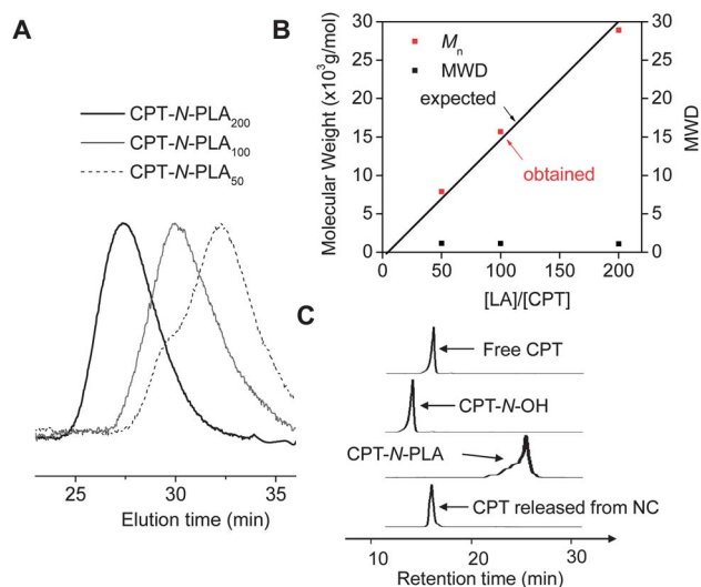
Fig. 2 (A) Overlay of GPC traces of CPT- N -PLA n ( n = 50, 100 and 200). (B) (BDI-EI)ZnN(TMS) 2 /CPT mediated ring-opening polymerization (ROP) of LA at various ratios of LA/CPT (MWD = molecular weight distribution). (C) HPLC analysis of CPT- N -OH initiated polymerization and release of CPT from CPT- N -PLA n NC. (HPLC traces from top to bottom: free CPT, CPT- N -OH, CPT- N -PLA, CPT released from CPT- N -PLA NC).
